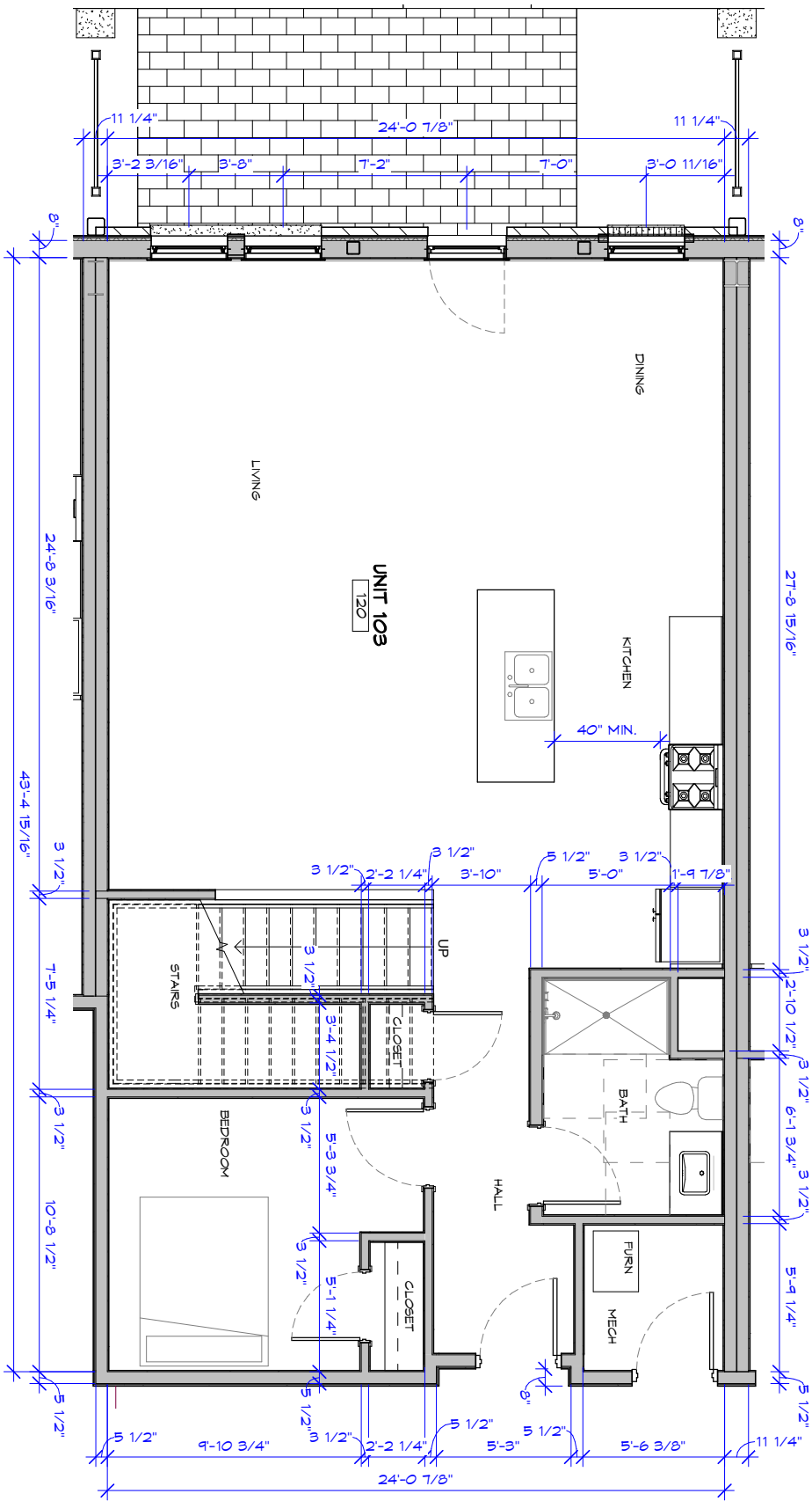
UNIT 103, 104 & 105 FIRST FLOOR PLAN
