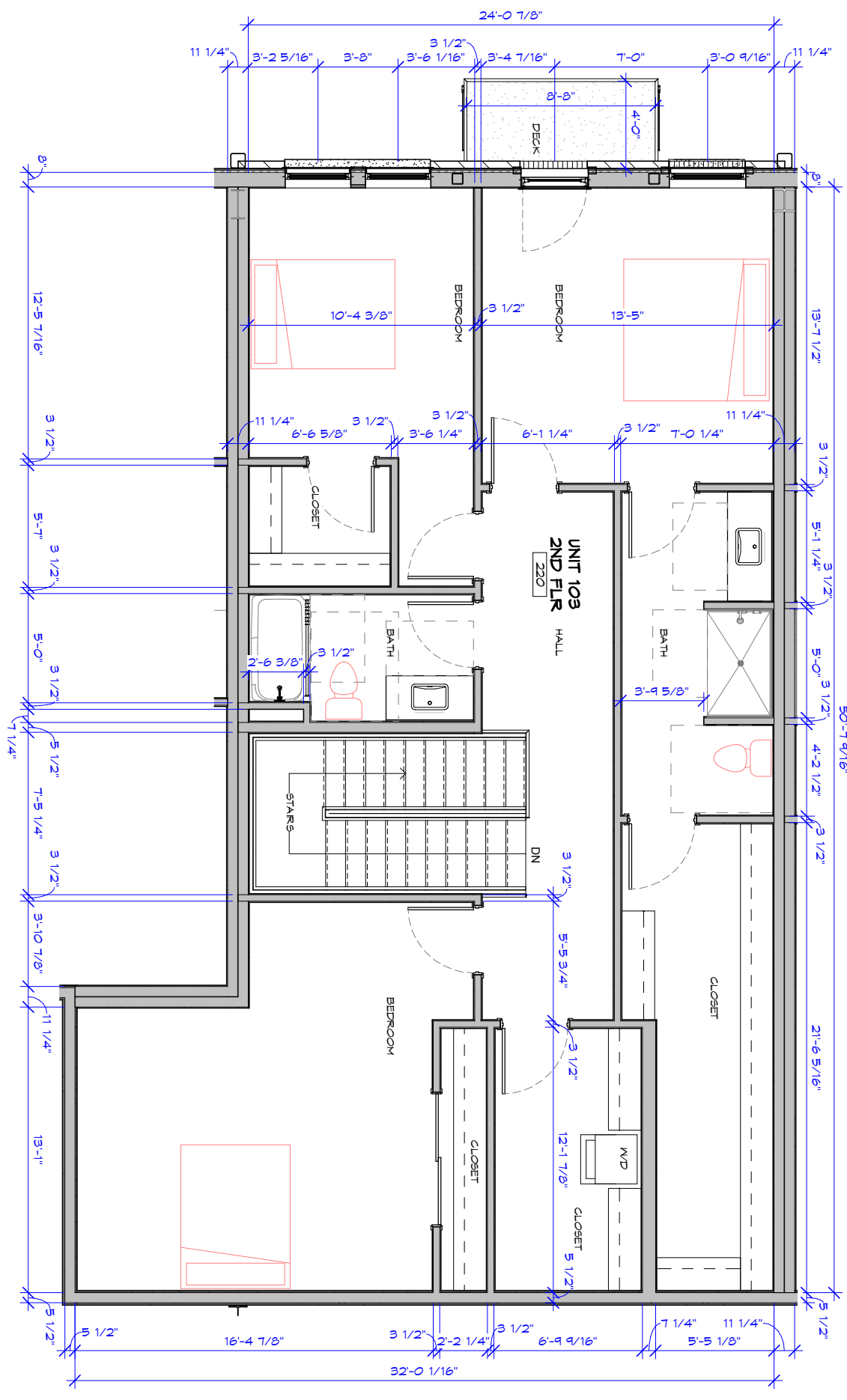
UNIT 103, 104 & 105 SECOND FLOOR PLAN
